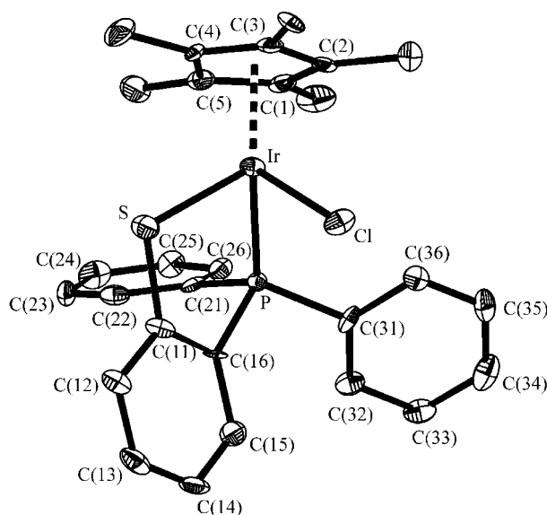
Figure 2. Molecular structure of [Ir(η 5 -C 5 Me 5 )(η 2 -2-Ph 2 PC 6 H 4 S)Cl] ( 3 ) with 50% probability ellipsoids and the labelling scheme; selected bond lengths [pm] and angles [°]: Ir–Cl 241.93(18), Ir–P 227.32(18), Ir–S 238.0(2); C(1)–Ir–C(3) 63.7(3), C(1)–Ir–C(4) 64.0(3), C(1)–Ir–Cl 126.9(2), C(1)–Ir–P 103.2(2), C(1)–Ir–S 143.0(2), C(2)–Ir–C(1) 37.6(3), C(2)–Ir–C(3) 38.2(3), C(2)–Ir–C(4) 63.0(3), C(2)–Ir–Cl 95.1(2), C(2)–Ir–P 127.0(2), C(2)–Ir–S 150.3(2), C(3)–Ir–Cl 94.5(2), C(3)–Ir–P 165.1(2), C(3)–Ir–S 112.3(2), C(4)–Ir–C(3) 37.1(3), C(4)–Ir–Cl 125.7(2), C(4)–Ir–P 145.7(2), C(4)–Ir–S 90.67(18), C(5)–Ir–C(1) 38.9(3), C(5)–Ir–C(2) 64.3(3), C(5)–Ir–C(3) 64.5(3), C(5)–Ir–C(4) 39.2(3), C(5)–Ir–Cl 157.9(2), C(5)–Ir–P 110.4(2), C(5)–Ir–S 104.5(2), P–Ir–Cl 88.02(6), P–Ir–S 82.42(7), S–Ir–Cl 89.45(8).
