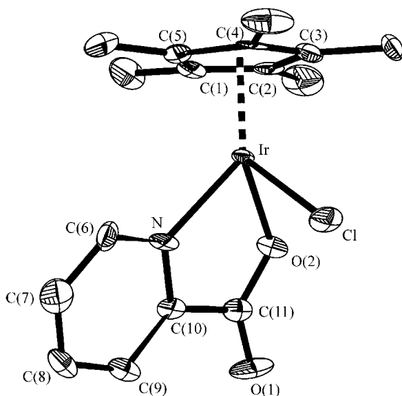
Figure 1. Molecular structure of [Ir(η 5 -C 5 Me 5 )(η 2 -C 5 H 4 N-2-CO 2 )Cl] ( 2 ) with 50% probability ellipsoids and the labelling scheme; selected bond lengths [pm] and angles [°]: Ir–Cl 239.97(15), Ir–N 208.8(7), Ir–O(2) 210.1(5), O(1)–C(11) 122.5(9), O(2)–C(11) 127.9(10); C(1)–Ir–C(2) 37.2(3), C(1)–Ir–C(3) 64.8(3), C(1)–Ir–Cl 160.8(3), C(2)–Ir–C(3) 39.2(3), C(2)–Ir–Cl 129.8(2), C(3)–Ir–Cl 96.92(19), C(4)–Ir–C(1) 66.2(3), C(4)–Ir–C(2) 65.5(3), C(4)–Ir–C(3) 39.1(3), C(4)–Ir–C(5) 39.2(3), C(4)–Ir–Cl 96.16(17), C(5)–Ir–C(1) 40.8(3), C(5)–Ir–C(2) 65.5(2), C(5)–Ir–C(3) 65.7(3), C(5)–Ir–Cl 128.03(18), C(11)–O(2)–Ir 117.7(4), N–Ir–C(1) 111.7(3), N–Ir–C(2) 144.5(3), N–Ir–C(3) 166.1(3), N–Ir–C(4) 127.0(3), N–Ir–C(5) 102.5(3), N–Ir–Cl 84.55(15), N–Ir–O(2) 77.0(2), O(1)–C(11)–O(2) 125.2(7), O(2)–Ir–C(1) 107.9(3), O(2)–Ir–C(2) 95.4(2), O(2)–Ir–C(3) 116.9(2), O(2)–Ir–C(4) 156.0(2), O(2)–Ir–C(5) 146.9(2), O(2)–Ir–Cl 85.02(14).
